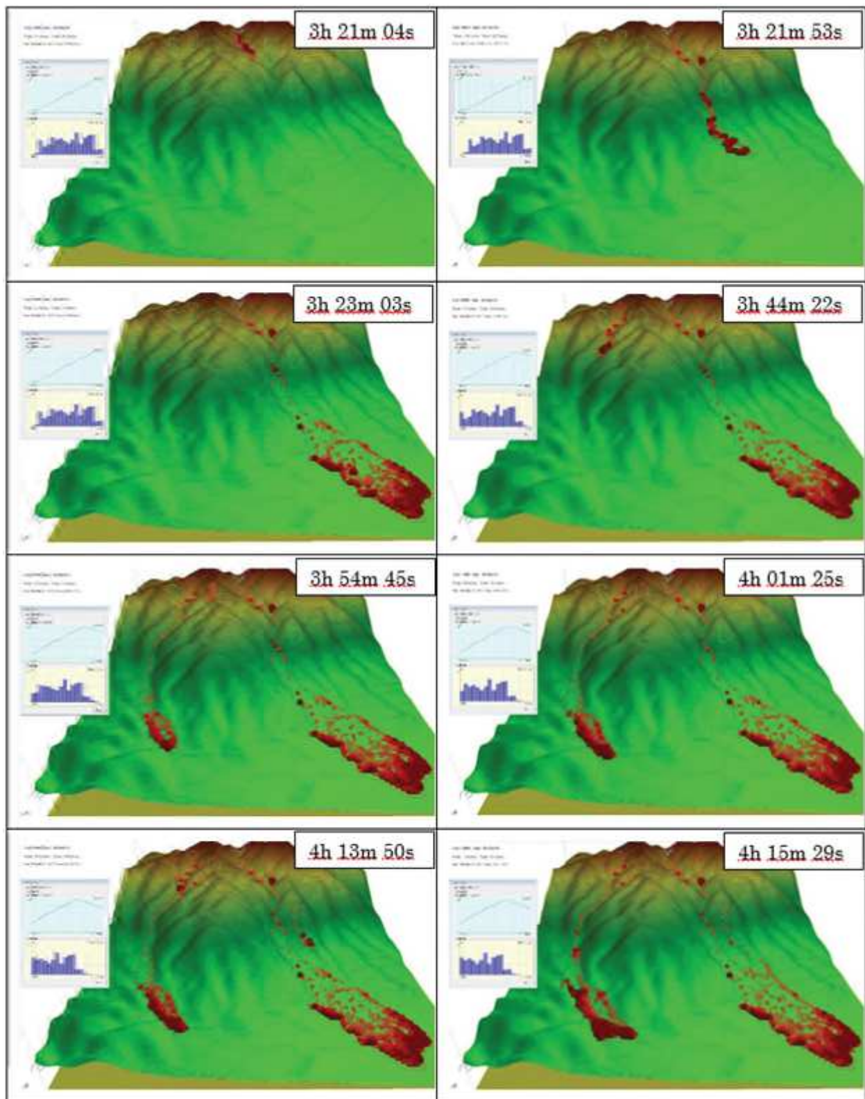
Fig.6 Landslide movement by LS-RAPID is presented together with 10 mm rainfall record and the excess pore pressure ratio.
