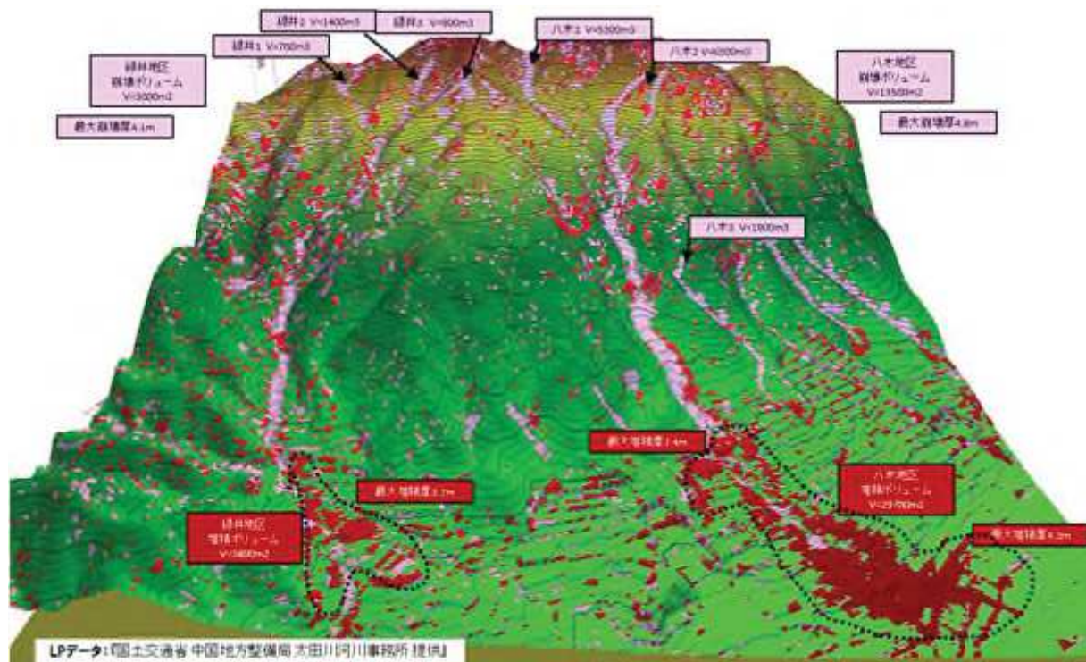
Fig. 5 Comparison of LS-RAPID simulation and Laser Profiler (LIDAR) before/after the disaster (By the Ohta-River Office of the Ministry of Land, Infrastructure, Transport and Tourism (MLIT))
