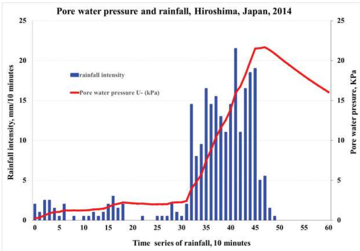
Fig. 4 Calculation of pore pressure ratio from rainfall intensity
