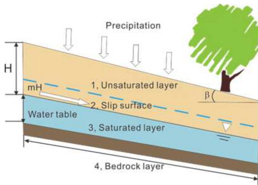
Fig. 3 Schematic illustrating the water infiltration the infinite slope (from Liao et al 2010)
